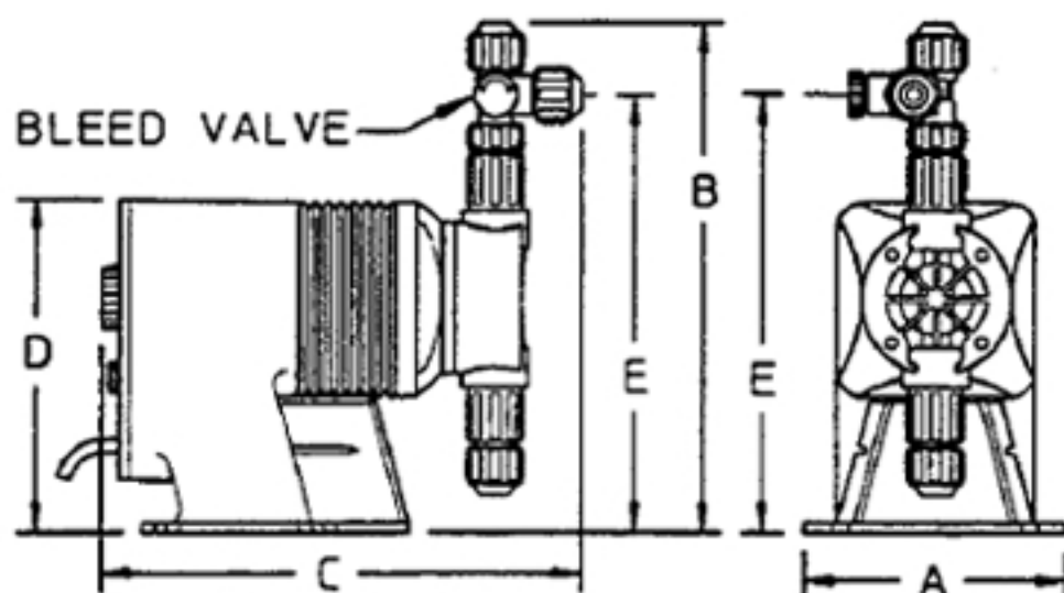
Series C Dimensions (inches)
