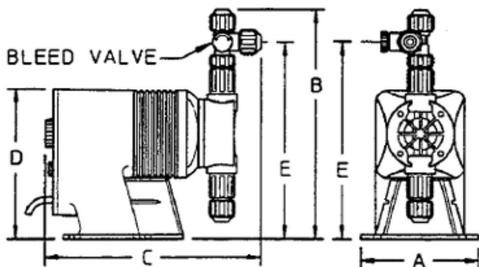
Series C PLUS Dimensions (inches)
