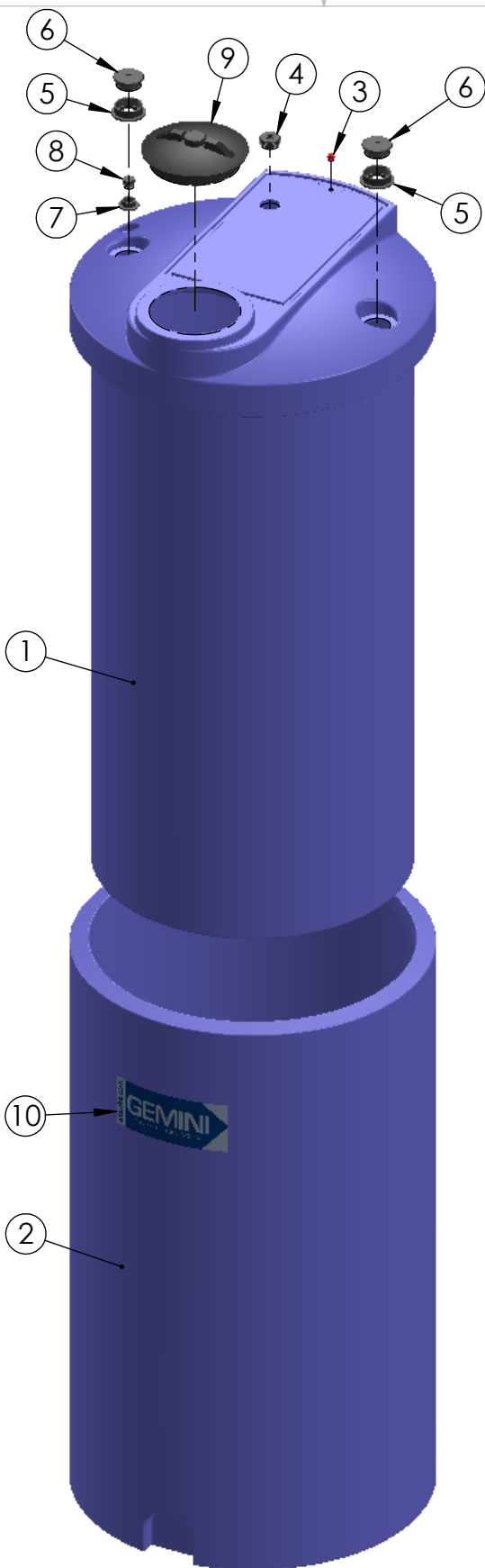
TRIMETRIC VIEW (EXPLODED)
