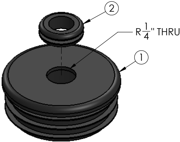
2" CAPLUG / GROMMET SUB-ASSY
