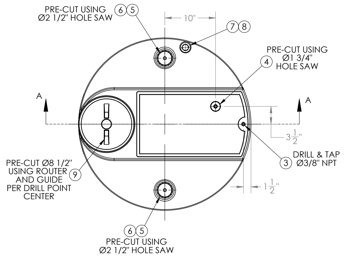
PLAN VIEW (ITEM DETAIL CALLOUTS PER TOP LEVEL BOM ON SHEET #1)
